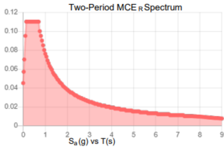
MCE_R Vertical Response Spectrum
